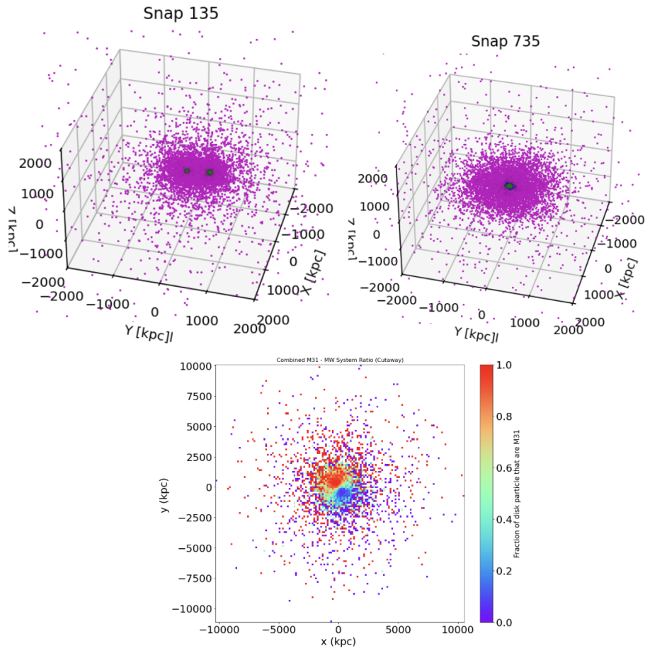
Figure 2. The two figures at the top are three dimensional plots of a sample of the particles before the merger(left) and after the merger(right). These visualize the investigation this project is doing into the shape of the remnant. The figure at the bottom is a histogram of the ratio of M31 to Milky Way particles. This visually represents the project's examination of the contributions from the two original galaxies to the final remnant.
